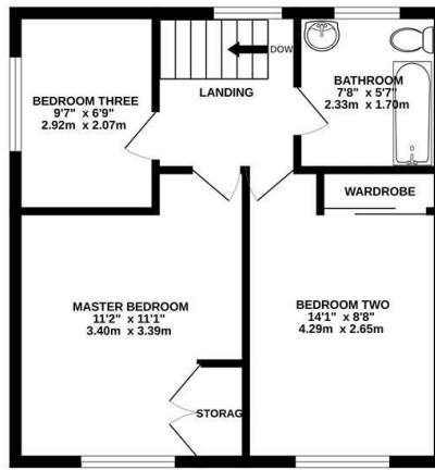
1ST FLOOR 445 sq.ft. (41.4 sq.m.) approx.
